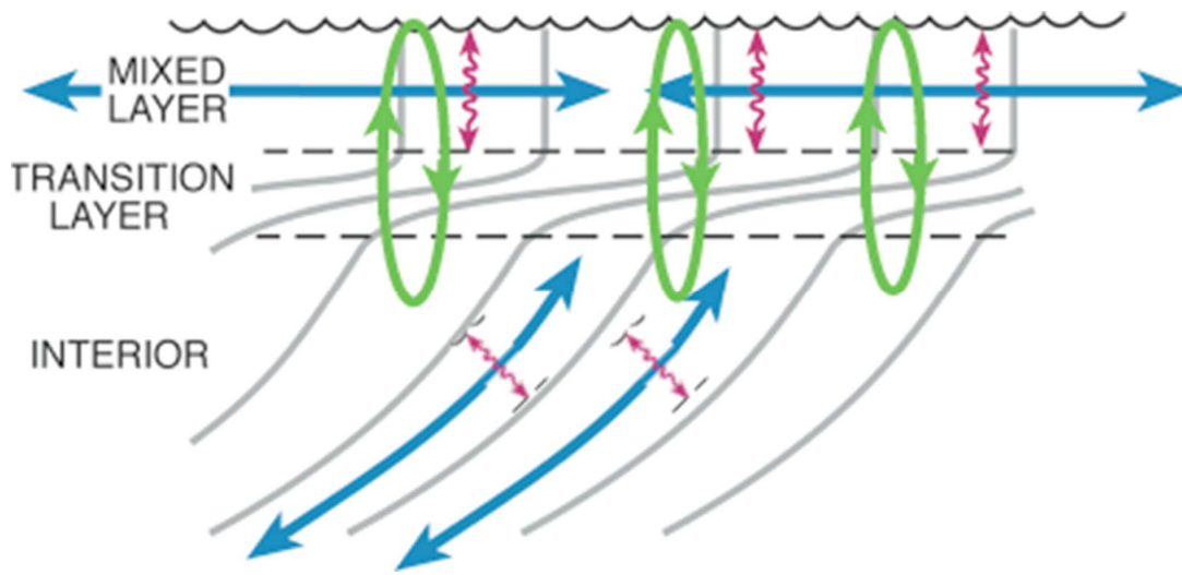
Figure 2. The oceanic motion at submesoscales (1-100 km, in green color) are effective in transferring heat, carbon dioxide, and other water properties from ocean surface to the deep ocean. Blue color represents motions at mesoscales (100-500km) transferring ocean properties mostly horizontally and red color represents mixing processes at scales less than 1 km (courtesy of R. Ferrari of MIT).
