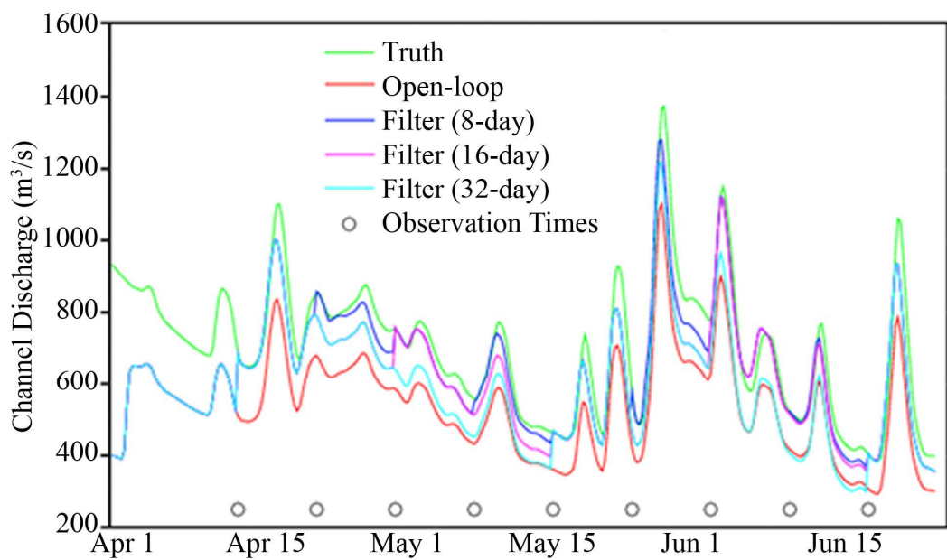
Figure 4. Discharge estimates from assimilating synthetic SWOT observations into a hydrodynamic model of the Ohio River for different repeat times (top; from Andreadis et al., 2007).
