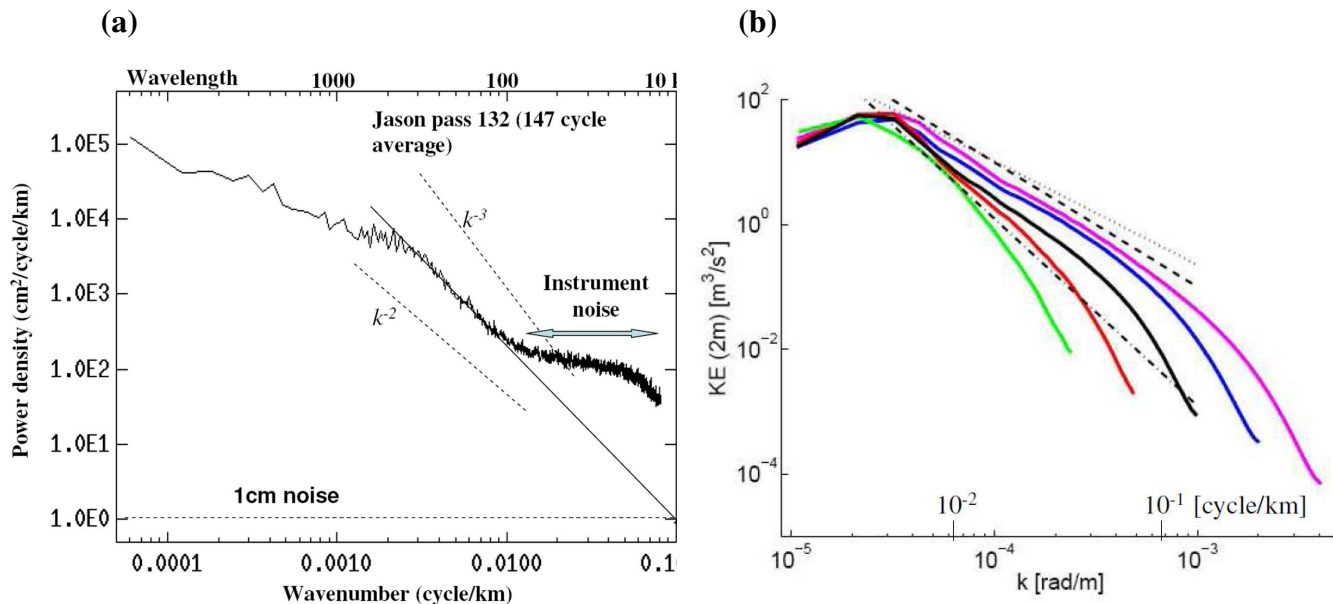
Figure 1 (a) Spectrum of sea surface height anomaly from Jason altimeter data (solid line). The two slanted dashed lines represent two spectral power laws with k as wavenumber. The horizontal dashed line represents the threshold of measurement noise at 1/km sampling rate. The slanting solid straight line represents a linear fit of the spectrum between 0.002 and 0.01 cycles/km. It intersects with the threshold noise level at 10 km wavelength. (from Fu and Ferrari, 2008). (b) Wavenumber spectra for simulated kinetic energy at 10- m depth. Straight lines indicate -5/3 (dotted), -2 (dashed), and -3 (dot-dash) spectrum slopes. The five other lines correspond to different simulations whose resolutions increase from 12 (green), 6 (red), 3 (black), 1.5 (blue) to 0.75 km (purple). (From Capet et al., 2008)
