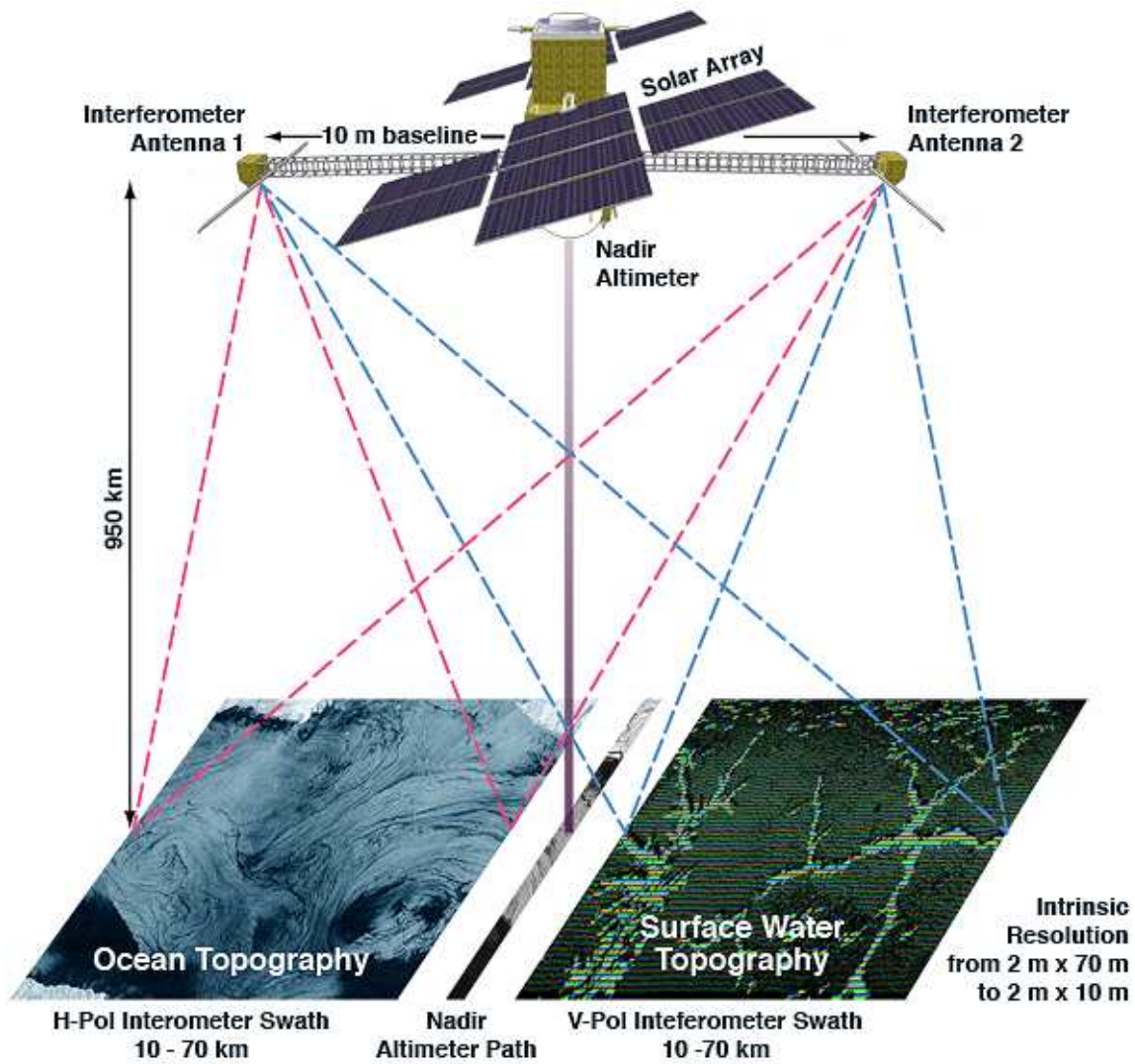
Figure 5. A schematic illustration of the measurement configuration of the SWOT Mission.
